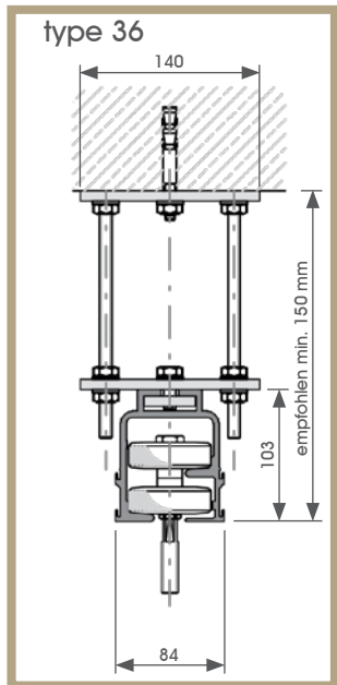
2-punts rail (type 36)
