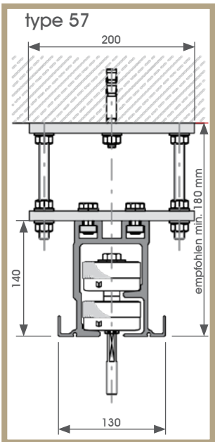
2-punts rail (type 57)
