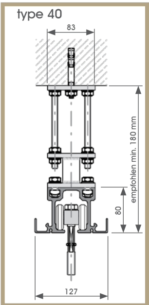
1-punts rail (type 40)
