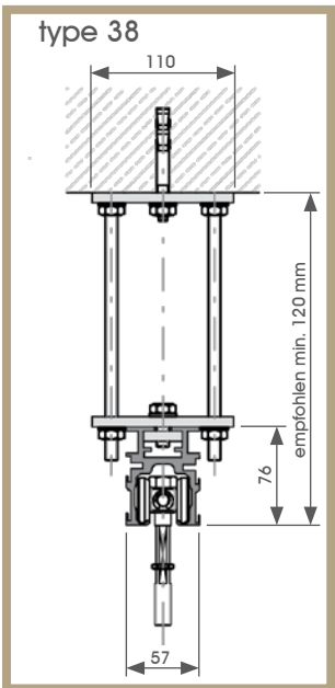
1-punts rail (type 38)
